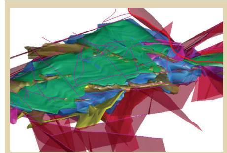
Mineralised bodies and fault system
